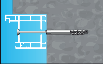
Ø 6 fixing with fastening
