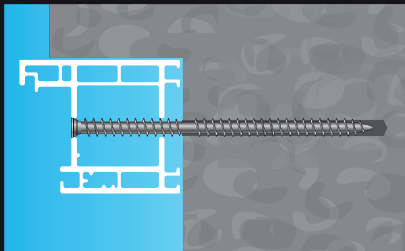
Ø 6.5 fixing with concrete screw
